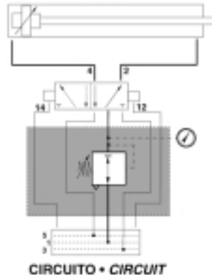
CIRCUITO • CIRCUIT
